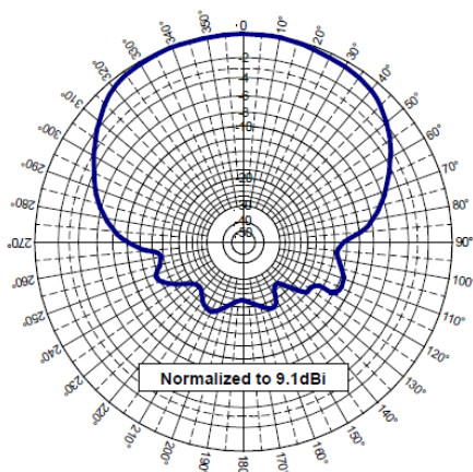
Elevation Pattern (Phi = 90°)
